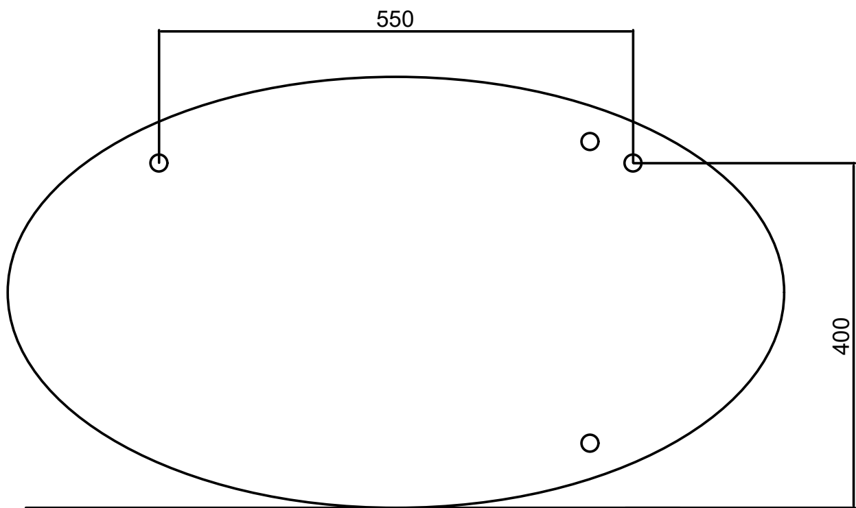
Horizontal Mirror Mounting Reference point
